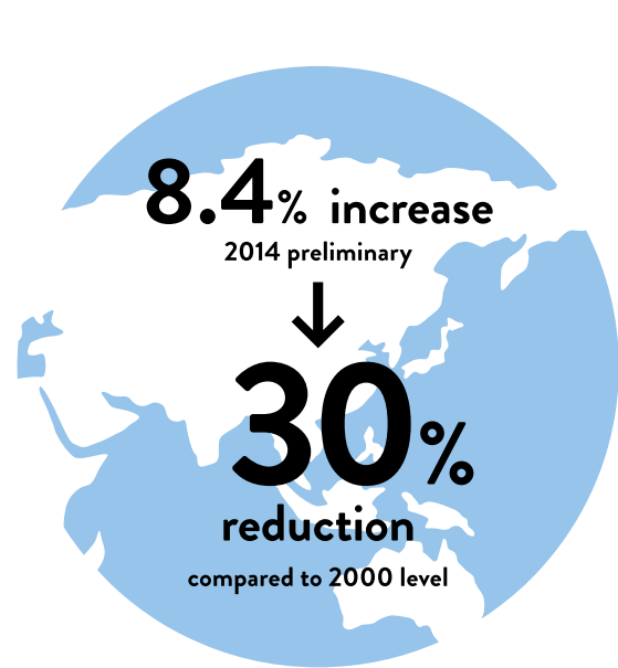
▶ Greenhouse Gas Emissions ◀
