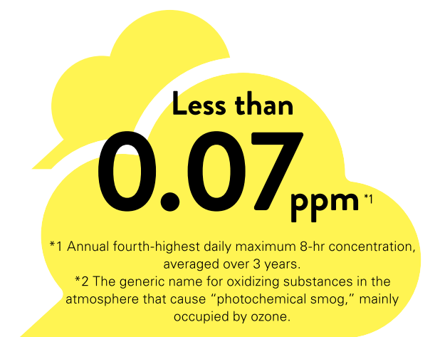
▶ Photochemical Oxidant *2 Concentration in All Monitoring Stations ◀
