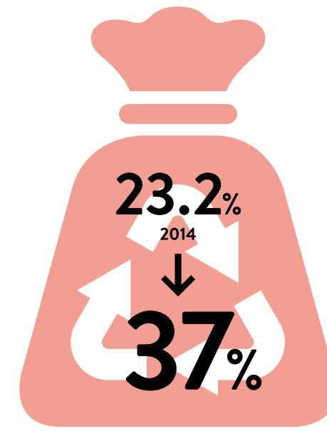
▶ Recycling Rate of Municipal Solid Waste ◀
