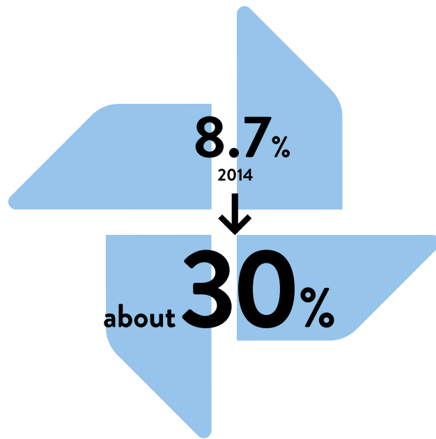
▶ Renewable Energy Target for Electricity Use ◀
