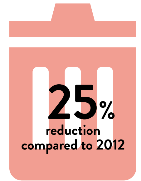
▶ Final Disposal Amount of Waste ◀
