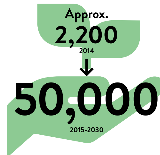
▶ Number of Participants in Field Work Programs ◀
